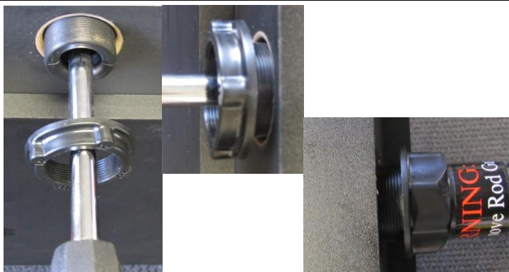
13. Slide bearing nut over handle & tighten 14. On rod side install Rod Guard Bearing and tighten fully
