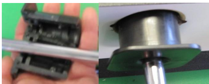
12. Take 2 bearing halves (#1 and #2) and connect them over rod and then place them into wall by aligning tabs with openings in the side of wall opening.
