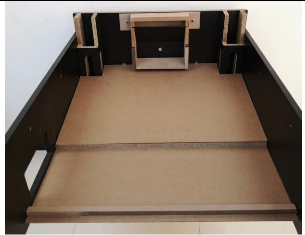
6b –Install Ball Return Board B (1)
