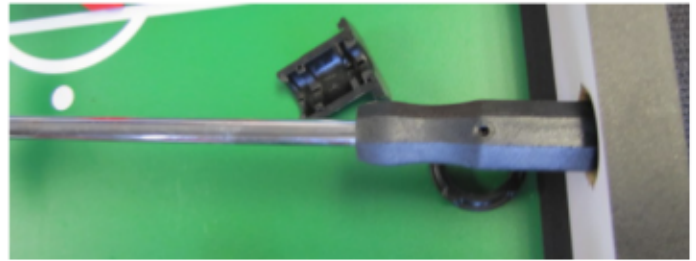
11. Guide handle through opening in near wall in proper position. Pull all the way in to allow other end of rod to clear far wall.
